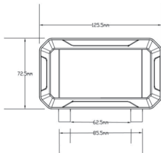
Figure 3-4 90T-H Front View Dimension
