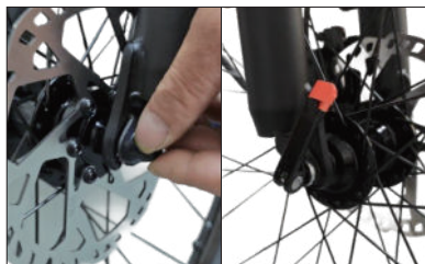
05 Install the front wheel onto the front fork, attach the protective screws, and lock the front wheel axle.
