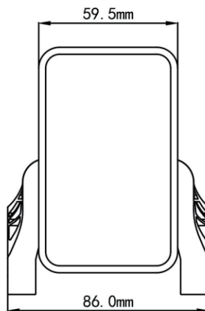
Figure 3-4 90T-V Front View Dimension
