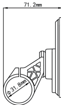
Figure 3-5 90T-V Side View Dimension
