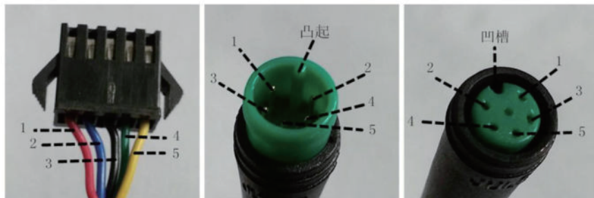
Controller connector
