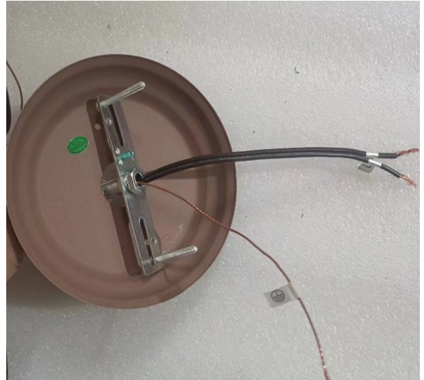
Step 5: Put it into the top plate as shown, and pass the wire.
