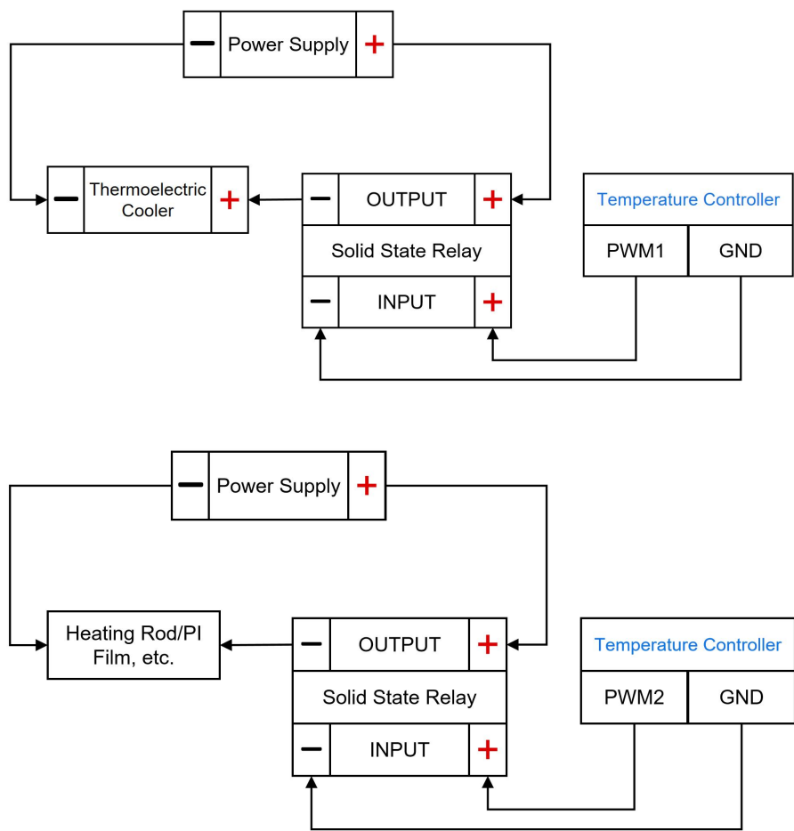
SSR wiring for cooling only (upper) and heating (lower)
