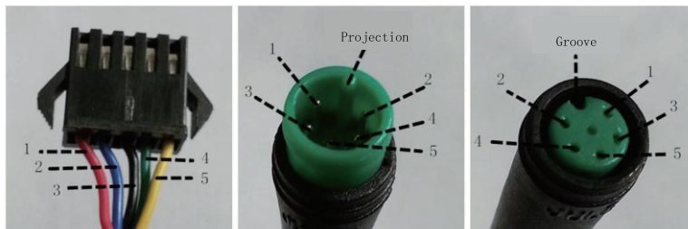
Controller connector
