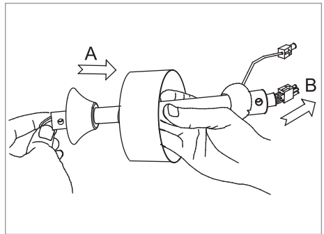
4. Let the downrod across the canopy, Magnet cover and coupler cover in the right direction, then put the power cord through downrod.
