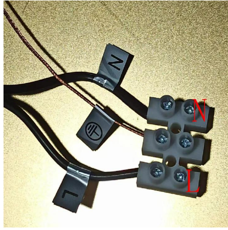
Step 4: Connect C to the user power cable with L, Note the distinction between N and L wire.
